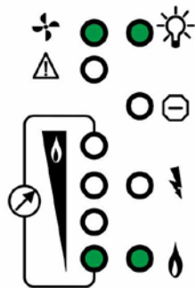
Flame detected Flame Signal over 5µA
