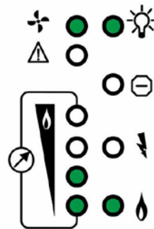
Flame detected Flame Signal over 10µA
