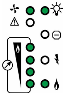
Flame detected Flame Signal over 20µA
